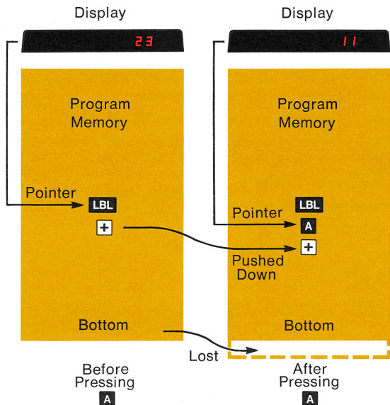
Figure 4-4. Editing Operations
